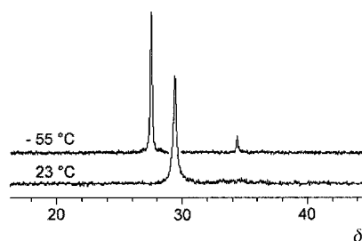
Figure 2. ^{31}\text{P} NMR spectrum of 8 at 23 and -55\text{ }^\circ\text{C} ( \text{CDCl}_3 ).
