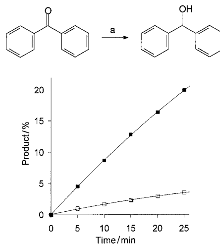
Figure 3. Product formation as a function of time for the transfer hydrogenation of benzophenone in the presence of catalyst P8 ( \blacksquare ) or P6 ( \square ). The data represent averaged values from two independent experiments; the errors are less than 0.4%. a) azeotropic \text{HCO}_2\text{H}/\text{NEt}_3 , \text{CH}_3\text{CN} , Ru catalyst, 70\text{ }^\circ\text{C} (benzophenone:Ru = 100:1).
