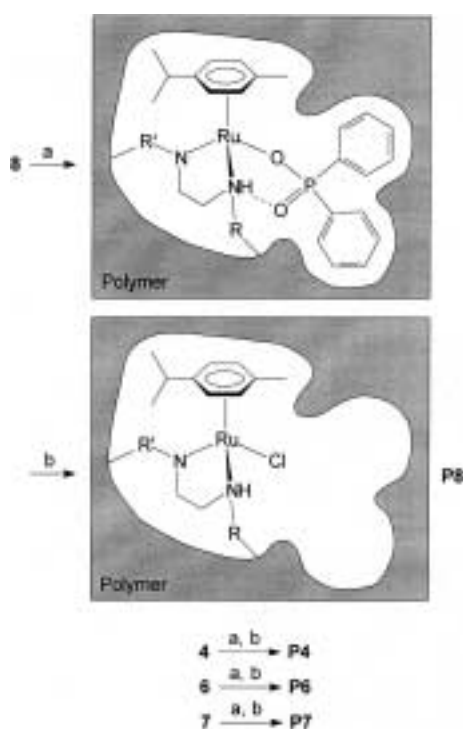
Scheme 4. Immobilisation of ruthenium complexes. a) EGDMA, \text{CHCl}_3 , V-70, 35\text{ }^\circ\text{C} , 20 h, then 65\text{ }^\circ\text{C} , 4 h; b) [\text{BnNEt}_3]\text{Cl} in MeOH (0.1M).
